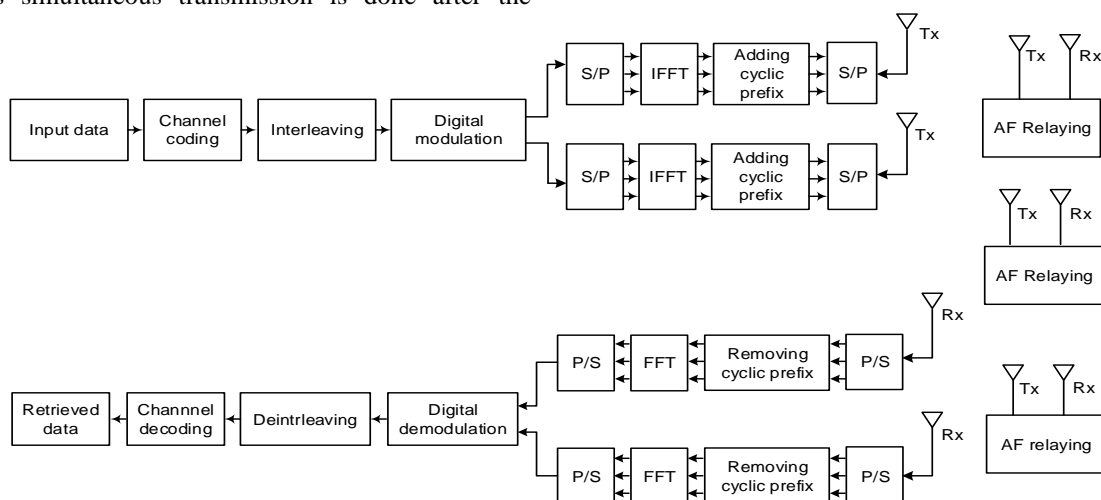
Fig. 1. Block diagram of Multiple Amplify and Forward Relayed Cooperative MIMO-OFDM system
