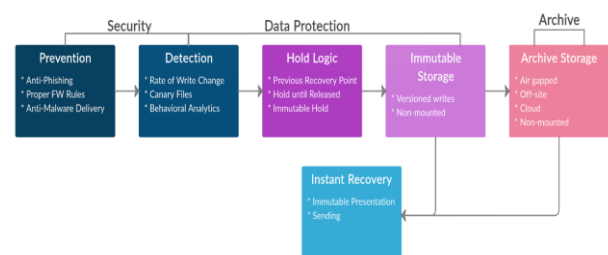
Fig 2. Architecture of Anti-Ransomware [14]
